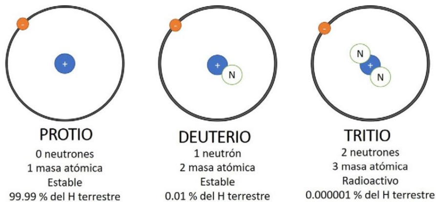
Figure 1: Hydrogen isotopes
